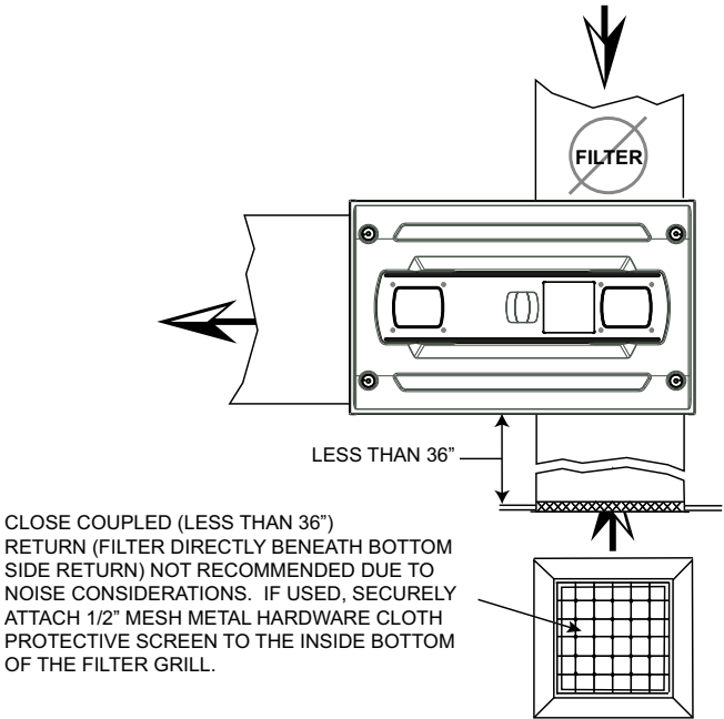
Figure 1. Horizontal upflow furnace with side return
