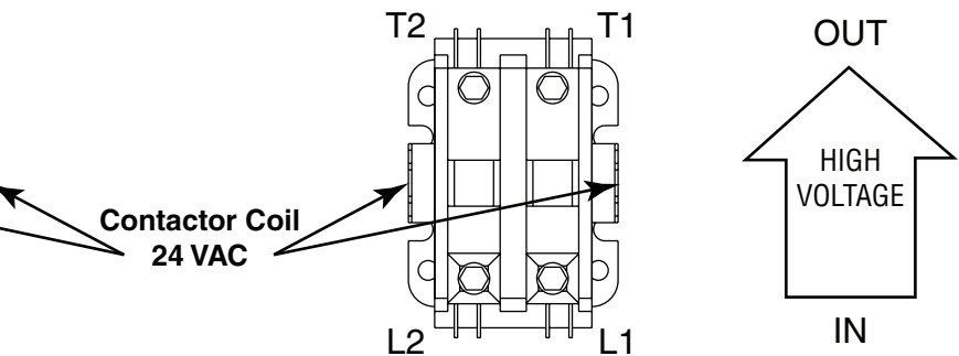
Double Pole Contactor (MS)*
