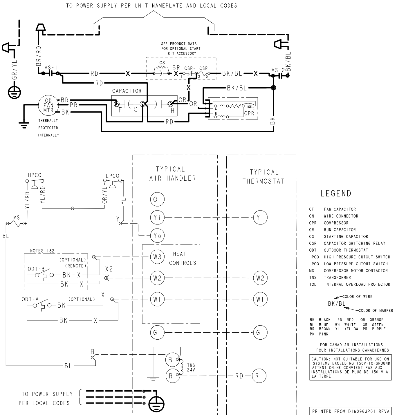
Figure 5. 060N Models
