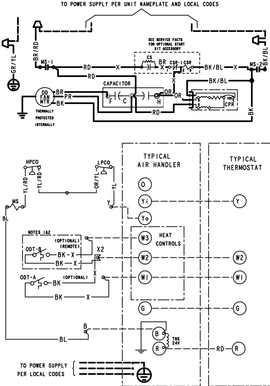
Figure 7. 060L Models
